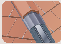
Uni-Vent Rapid Ridge/Hip & Continuous Hip Systems
