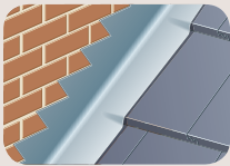
Wakaflex Rapid Flashing
